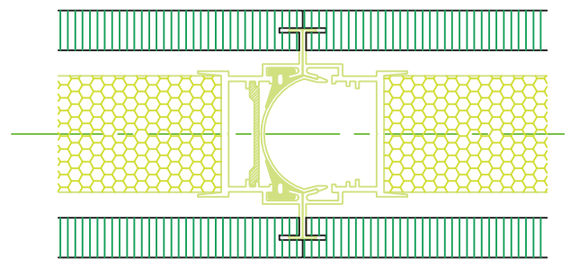
particolare nodo profili nascosti junction detail of hidden profile
