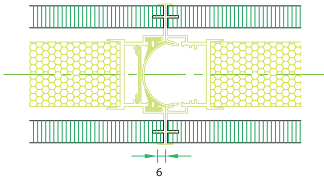
particolare nodo profili in vista junction detail of visible profile
