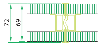
nodo con profili in vista junction detail of visible profile
